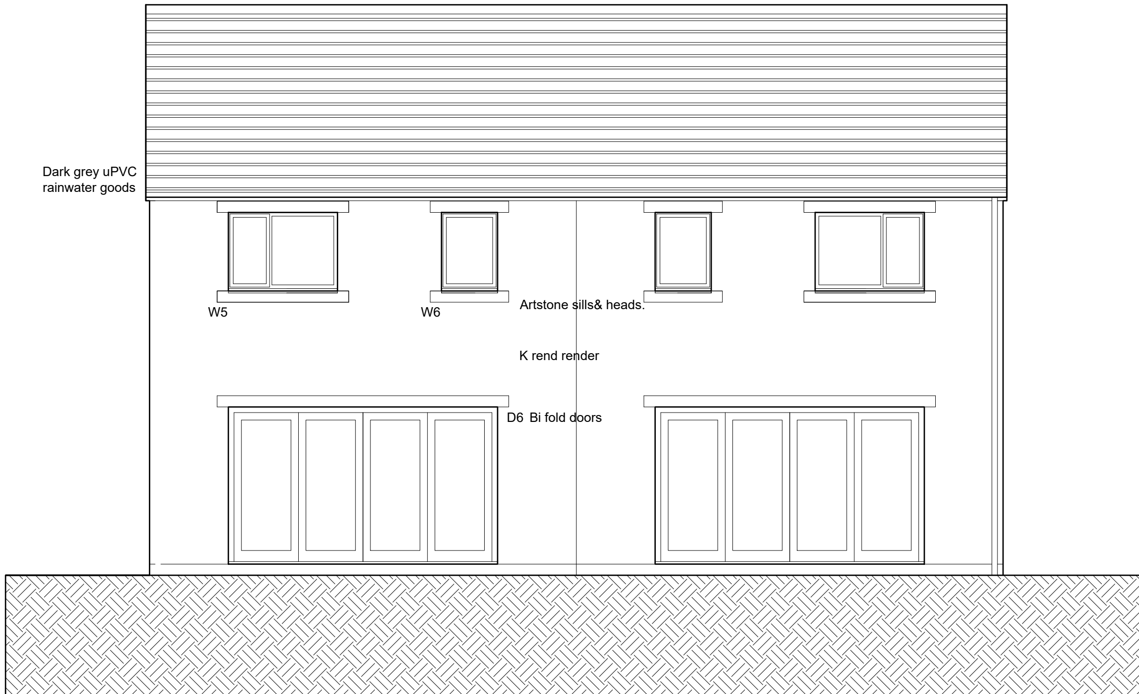
REAR ELEVATION
