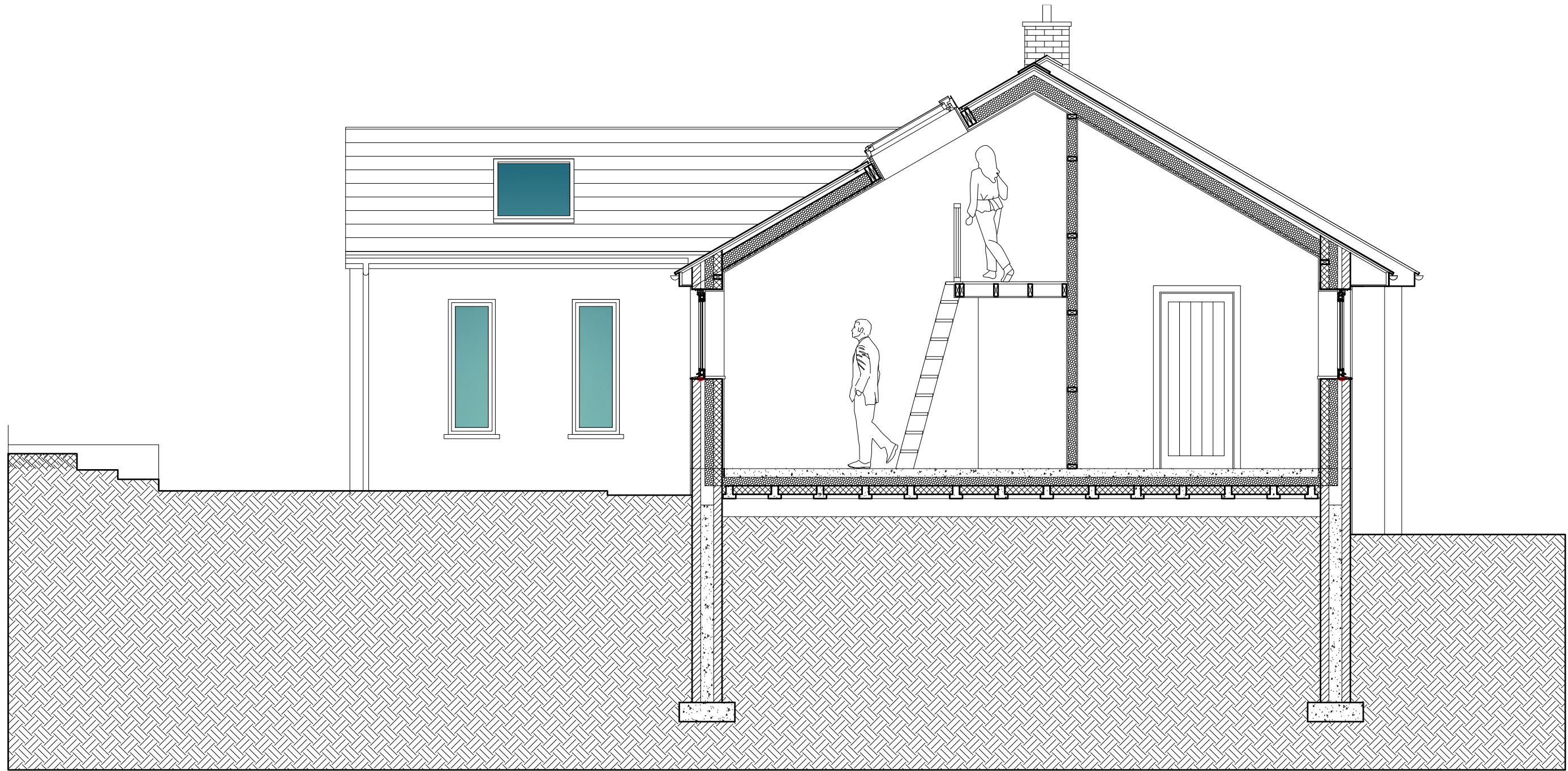
PROPOSED SECTIONAL ELEVATION
