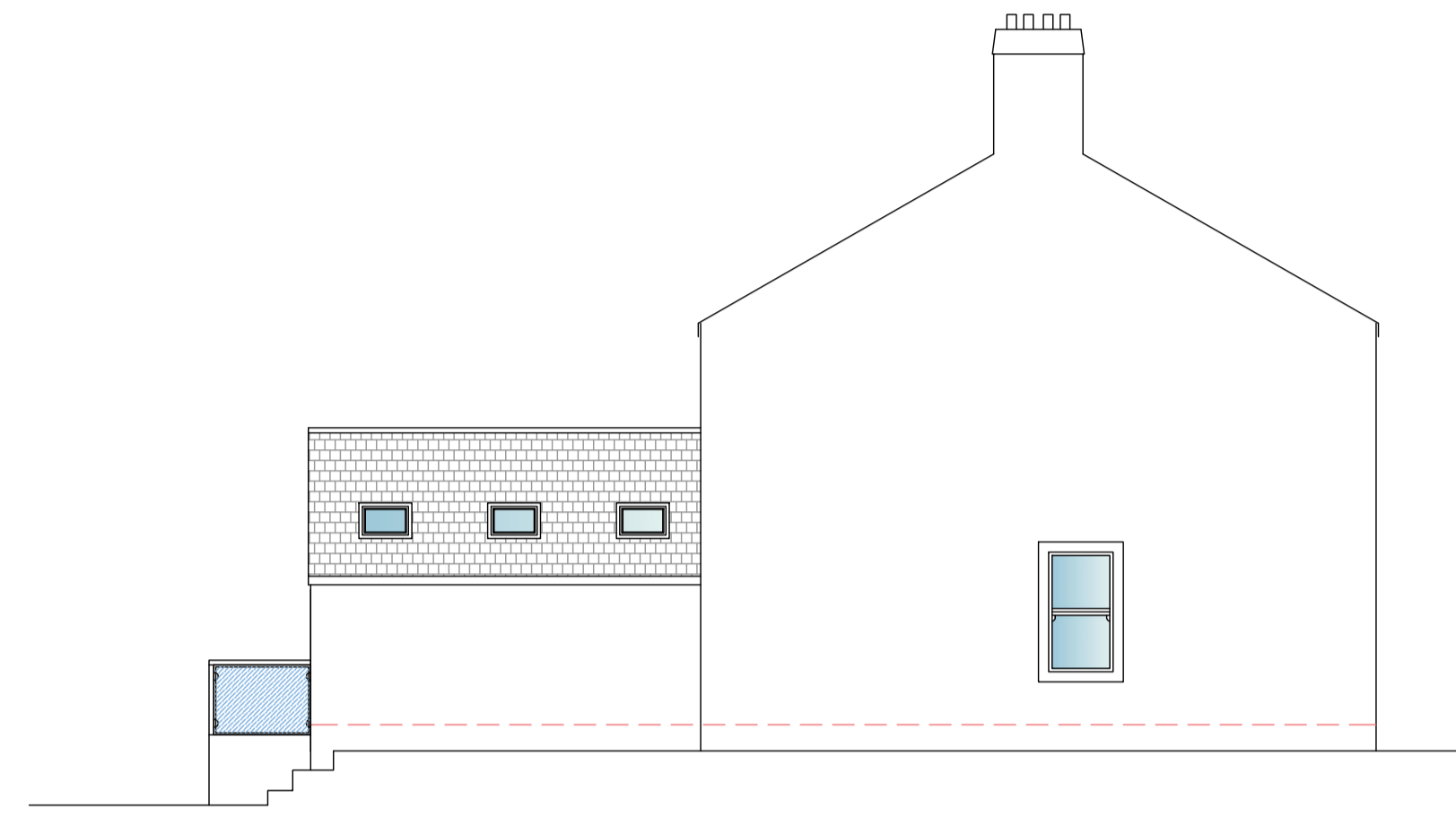
Side Elevation (View looking through Attached Property)
