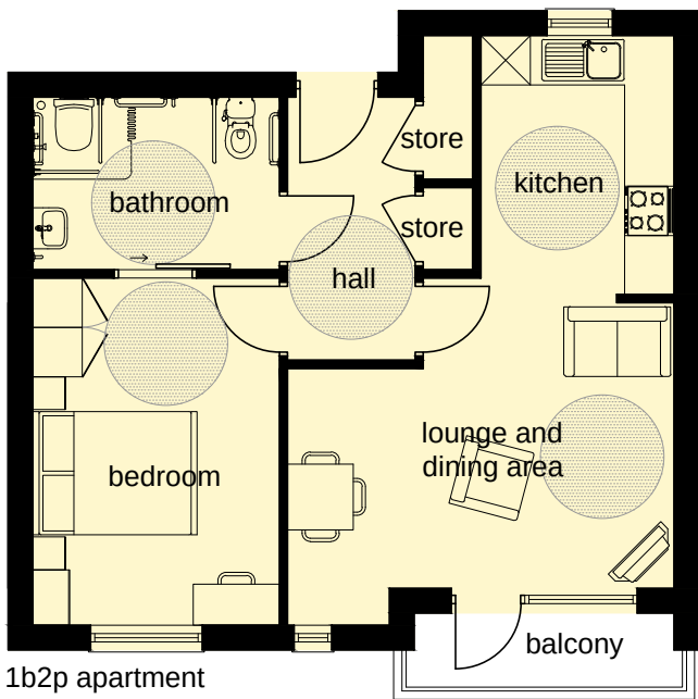
Apartment plans scale 1:100
